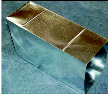
16.5" x 20.25" x 48" Sheet Metal Plenum with 2" Duct Liner, R8 Lined
