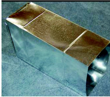
16.5" x 20.25" x 48" Sheet Metal Plenum with 1" Duct Liner
